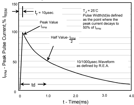
Fig.3 - Test Pulse Waveform
