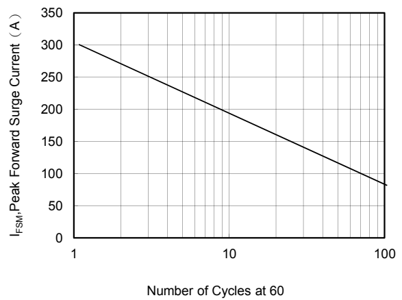
Fig.6 - Maximum Non-repetitive Forward
