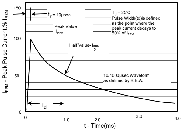
Fig.3 - Pulse Waveform
